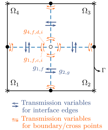
Figure 1: Example of domain decomposition ( 2 \times 2 configuration) with the transmission variables.
