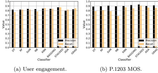
Figure 4: Prediction of user engagement and P.1203 MOS.
