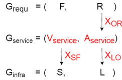
Fig. 4: Roles of the variables in graphs matching
