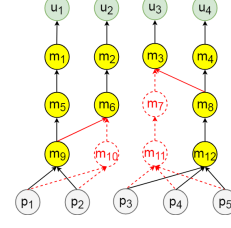
Fig. 5: A derivative G_M of G_U
