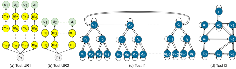
Fig. 6: Tests inputs
