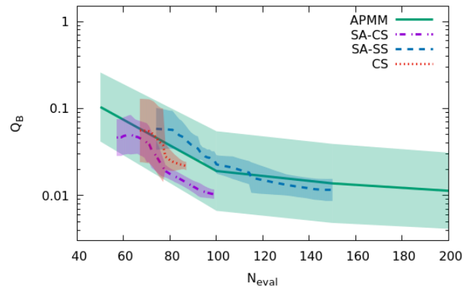
Figure 9: Test-case 1-a: Cost comparison between APMM and three SABBA variants.
