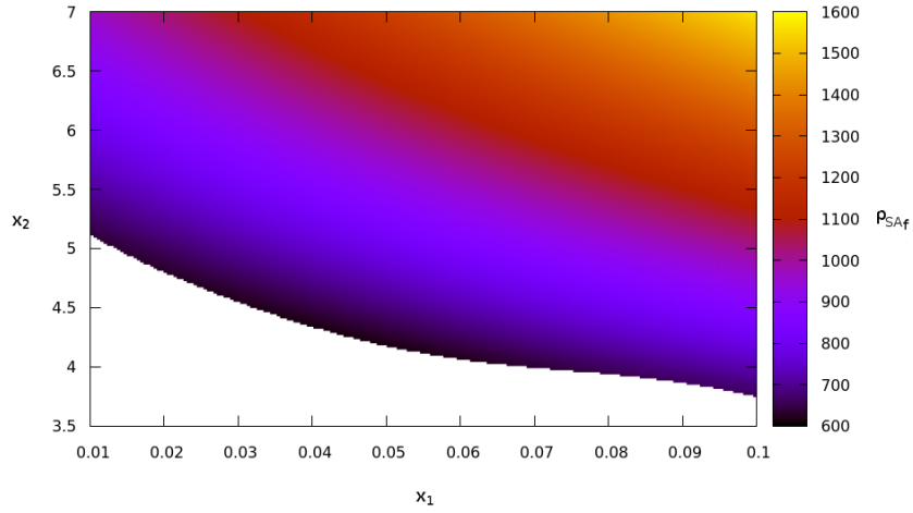
Figure 22: Final SA model, representing \rho_{SA_f}(\mathbf{x}) where the constraint \rho_{SA_g}(\mathbf{x}) \leq 473.15 K is satisfied.
