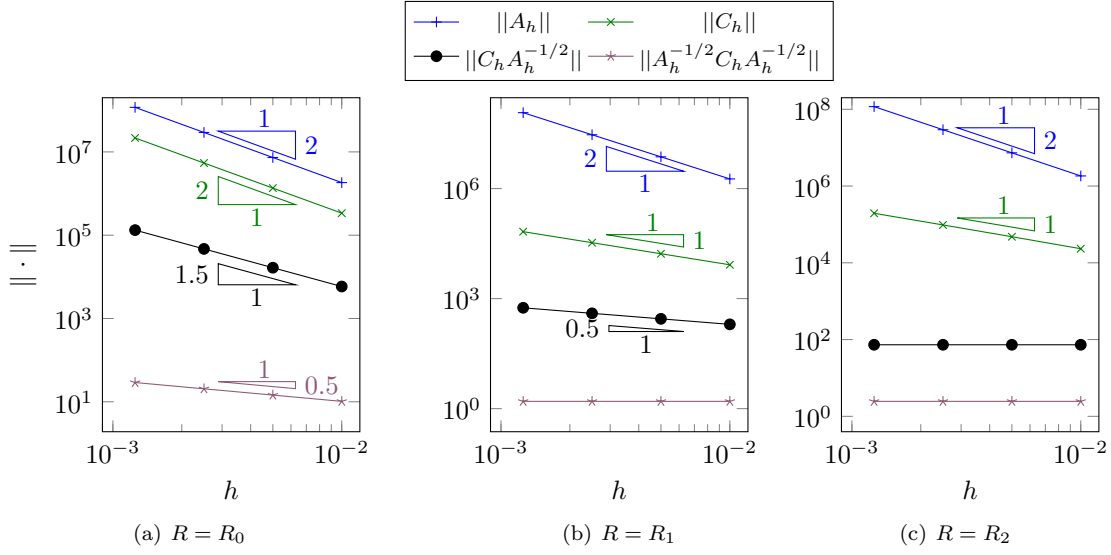
FIGURE 1. Norms of A_h , C_h , C_h A_h^{-1/2} and A_h^{-1/2} C_h A_h^{-1/2} with respect to h with \sigma = 1 on a uniform mesh of [0, 1] using fourth order finite elements.
