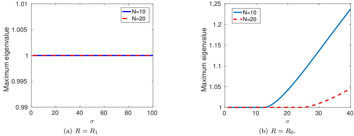
FIGURE 6. Evolution of the largest eigenvalue amplitude w.r.t. \sigma , N = 10, 20 .
