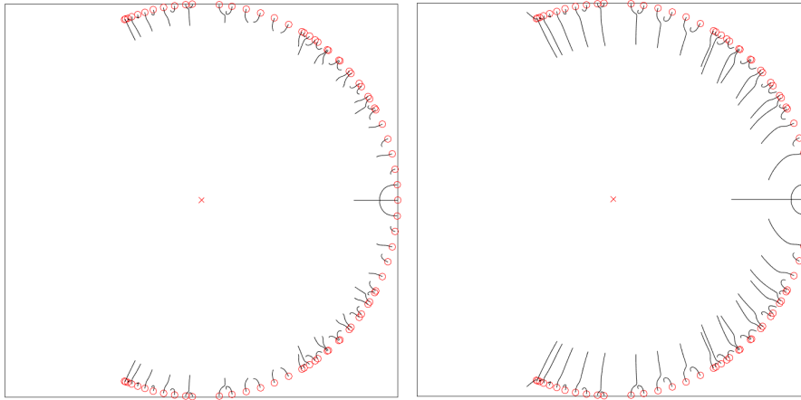
FIGURE 7. Trajectories of the eigenvalues of system (67) in the complex plane (with N = 10 and R = R_0 ). Left: \sigma varies between 0 and 10. Right: \sigma varies between 0 and 20. Note that for \sigma = 0 the eigenvalues are all located on the unit circle and their exact location is represented by circles. For \sigma \leq 10 no eigenvalue is of absolute value greater than one. For \sigma = 20 two eigenvalues are of absolute value greater than one .
