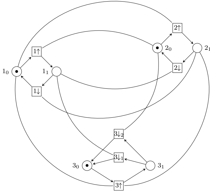
Fig. 4 CPN encoding of the BN of Fig. 1 \langle f_1(x) = \neg x_2, f_2(x) = \neg x_1, f_3(x) = \neg x_1 \wedge x_2 \rangle and configuration 000
