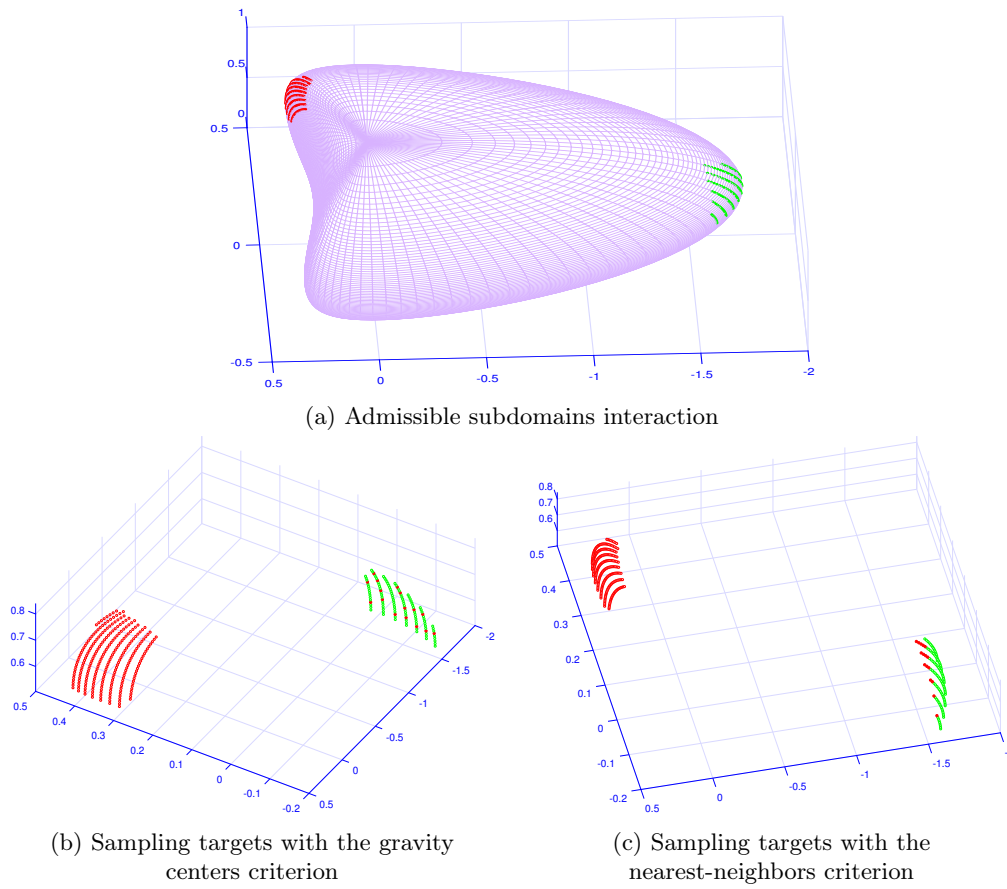
Figure 2: Surface from [2], with admissible subdomains created with \eta = 0.15 .
