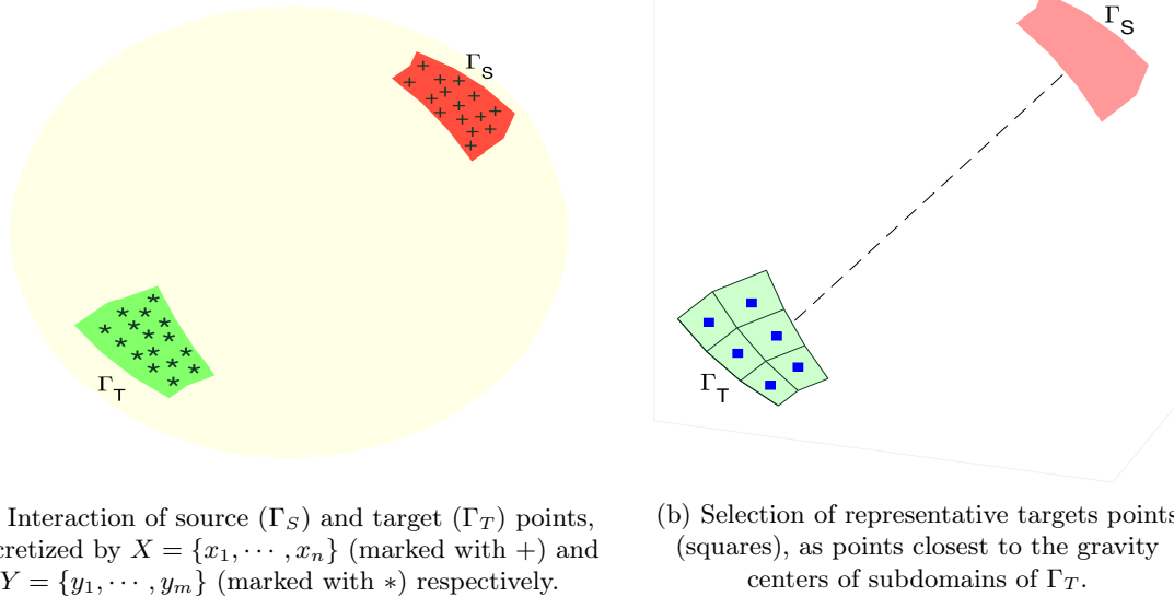
Figure 1: Interaction of distant subdomains on a sphere, and selection of representative target points.
