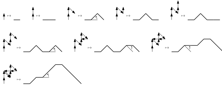
FIGURE 4. An example of the raising process describing the map \psi on the 3-step model.
