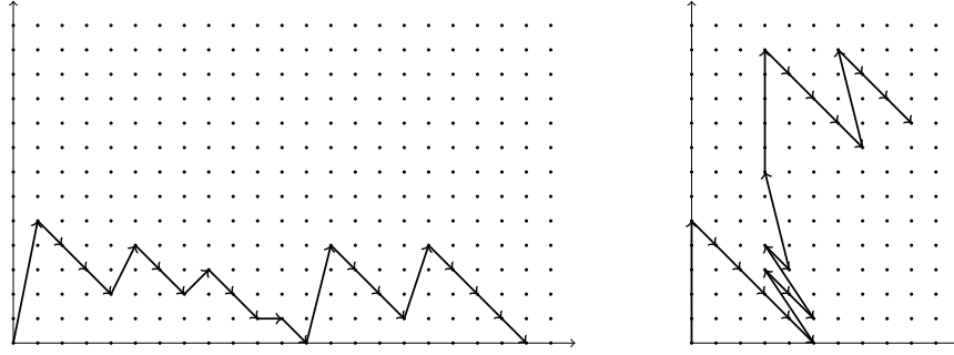
FIGURE 3. An example of a Łukasiewicz walk (left) and of the corresponding p -tandem word (right), for p = 5 and length 21.
