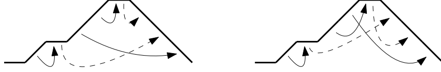
FIGURE 5. The example of Figure 4 showing the different pairings from the raising algorithm (left) and Eu, Fu, Hou, and Hsu's algorithm (right). Pairings indicated with solid lines come from 2b in the raising algorithm or the second pass of Eu, Fu, Hou, and Hsu's algorithm while pairings indicated with dashed lines come from 2c or the third pass.
