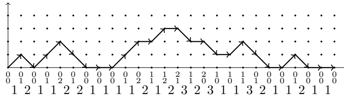
FIGURE 1. An example of a Motzkin walk (above) and of a Yamanouchi word (bottom), both of length 25, associated with one another by the maps \phi and \psi .
