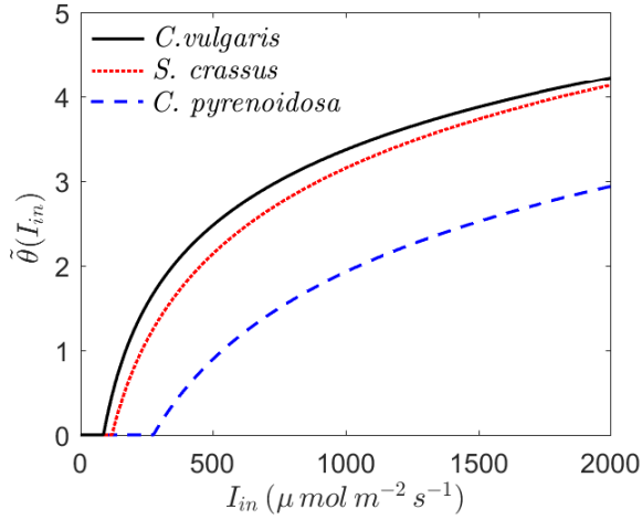
Figure 6: Critical optical depth \tilde{\theta} as a function of the incident light I_{in} for three different microalgae species. Kinetic parameters are taken from Table 2.
