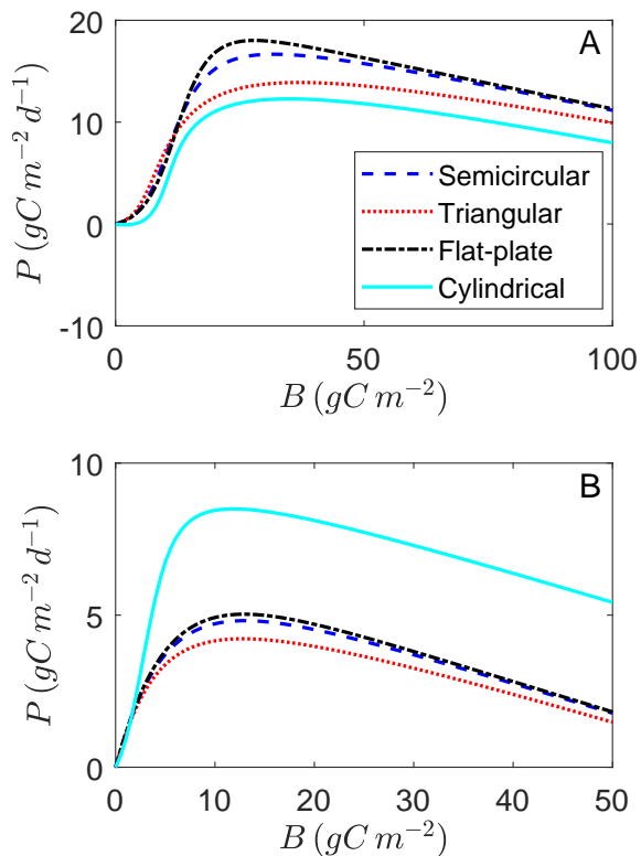
Figure 9: Productivity as a function of the biomass concentration per illuminated surface. A. I_{in} = 1000 \mu\text{mol m}^{-2} \text{s}^{-1} B. I_{in} = 50 \mu\text{mol m}^{-2} \text{s}^{-1} . We consider p given by (25) with the kinetic parameters of C. vulgaris given in Table 2. The other parameters are taken to be k = 0.2 \text{m}^2 \text{gC}^{-1} , m = 0.1 \text{d}^{-1} , and K_{bg} = 0 .
