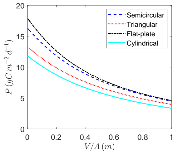
Figure 10: Maximal productivity as a function of V/A . p is given by (25) with kinetic parameters of C. vulgaris given in Table 2. Other parameters are taken to be I_{in} = 1000 \mu\text{mol m}^{-2} \text{s}^{-1} , k = 0.2 \text{m}^2 \text{gC}^{-1} , m = 0.1 \text{d}^{-1} , K_{bg} = 10 \text{m}^{-1} .
