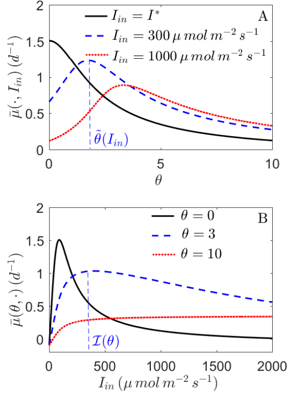
Figure 5: A. Plot of the AGR as a function of the optical depth for three different values of the incident light. B. Plot of the AGR as a function of the incident light intensity for three different values of the optical depth. We consider p given by (25) with the kinetic parameters of C. vulgaris given in Table 2 and m = 0.1 d^{-1} .
