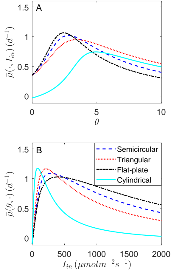
Figure 8: Plots of the AGR for different shapes of the PBR. A. I_{in} = 500 \mu mol m^{-2} s^{-1} is fixed. B. \theta = 3 is fixed. We consider p given by (25) with the kinetic parameters of C. vulgaris given in Table 2 and m = 0.1 d^{-1} .
