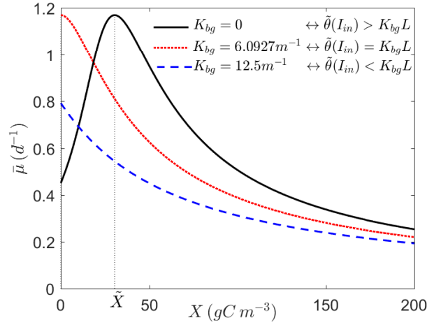
Figure 7: Plot of the AGR as a function of X . We consider p given by (25) with the kinetic parameters of C. vulgaris given in Table 2. The other parameters are taken to be I_{in} = 500 \mu mol m^{-2} s , k = 0.2 m^2 gC^{-1} , L = 0.4 m , and m = 0.1 d^{-1} .
