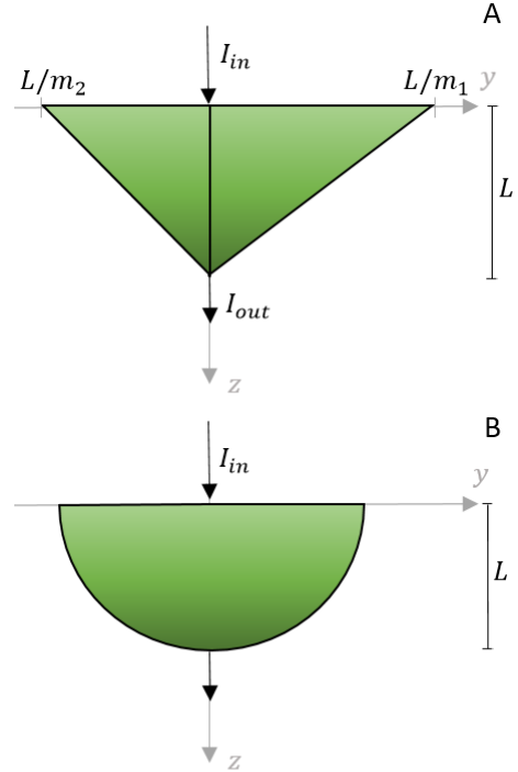
Figure 2: Schematic representation of a cross section through a cylindrical horizontal PBR. A. Triangular cylinder. The base measures L(1/m_1 + 1/m_2) and the height L . B. Semi-circular cylinder of radius L .
