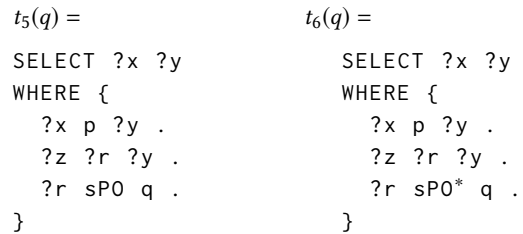
Figure 5: Queries expressed with respect to ontological expressions (sPO stands for rdafs:subPropertyOf ).
