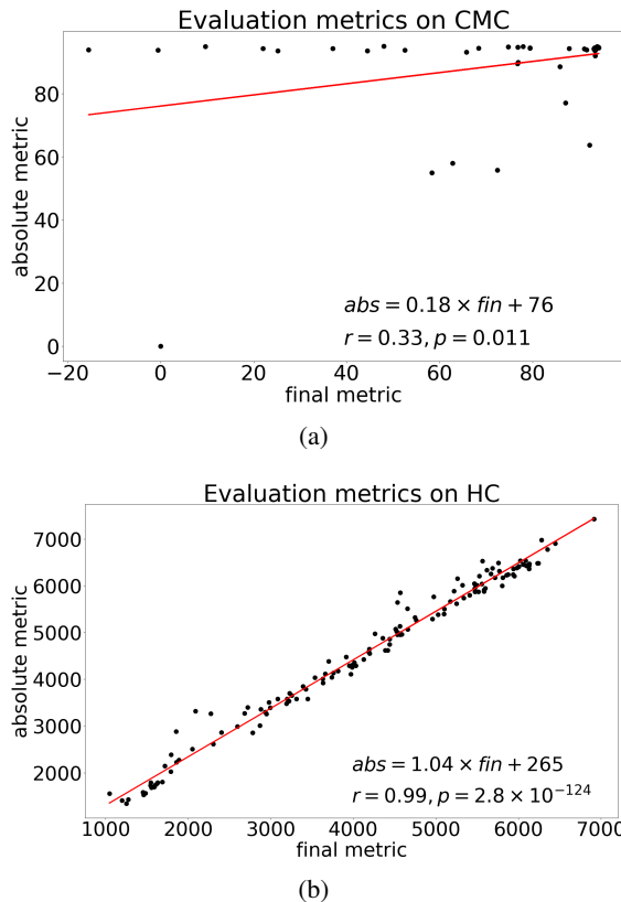
Figure 4. Correlation of the two metrics of performance on (a) CMC and (b) HC. The equations of the lines of best fit (in red), the Pearson coefficients r and their associated p -values p are provided.
