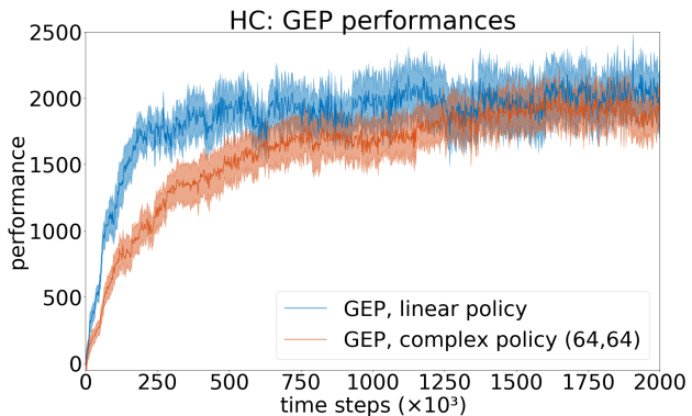
Figure 7. Performance of GEP for a linear and a policy with two hidden layers of (64,64) neurons.
