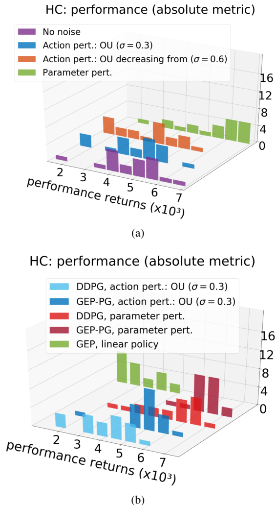
Figure 6. Absolute metric in HC for the various algorithms.(a) shows the influence of undirected exploration with perturbations on performance. (b) show the performances of GEP, DDPG and their combination GEP-PG on HC.
