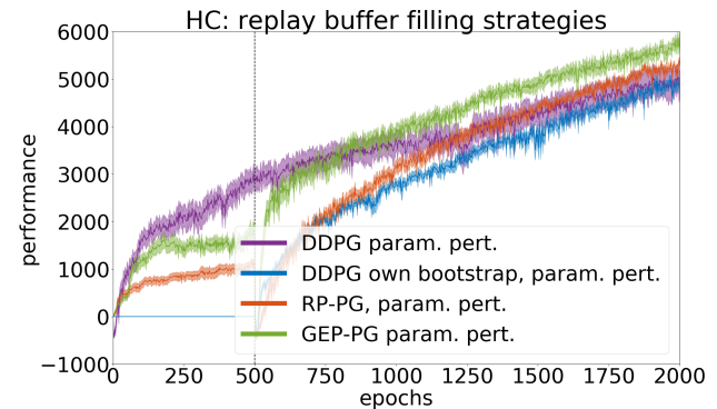
Figure 10. Influence of various exploration strategies to initialize DDPG’s replay buffer on GEP-PG performance. In the second curve, the parameter perturbation exploration of DDPG is used. In the exploration phase ( < 500 epochs), the networks are not updated. In the exploration phase of the third and fourth curves, Random Policy Search (RP) and Goal Exploration Process (GEP) are used respectively.
