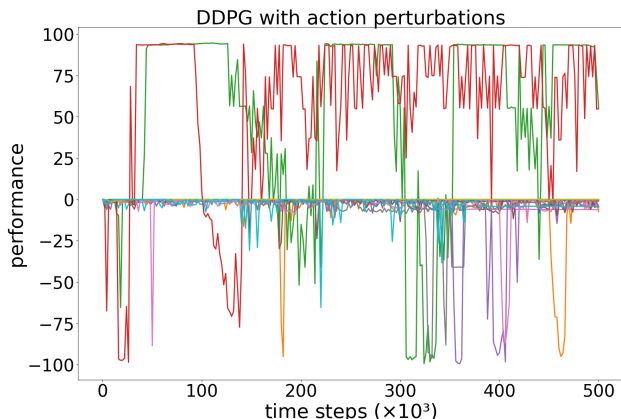
Figure 5. Twenty individual runs of DDPG OU(0.3) on CMC
