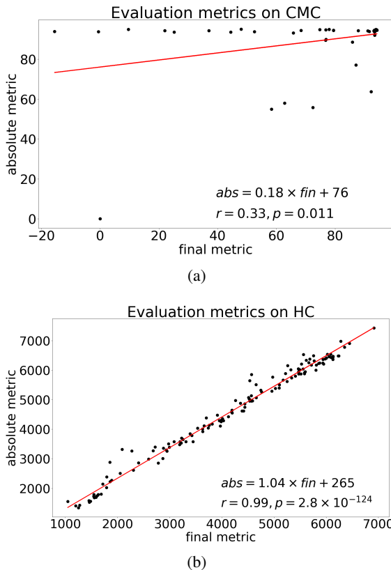
Figure 4. Correlation of the two metrics of performance on (a) CMC and (b) HC. The equations of the lines of best fit (in red), the Pearson coefficients r and their associated p -values p are provided.
