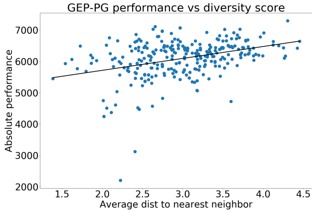
Figure 9. GEP-PG performance as a function of the buffer’s diversity measure. The diversity measure is computed as the average distance to the nearest neighbor in outcome space. It is normalized by the expected value of this measure in the case of a uniform distribution of outcomes. This normalization makes the measure insensitive to the number of considered samples (here through the size of the buffer).
