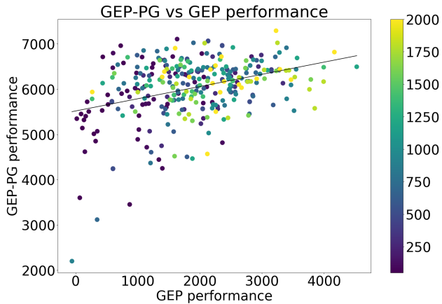
Figure 8. GEP-PG performance as a function of the GEP buffer performance. The GEP performance is evaluated by replaying 100 times the best policy found by GEP. Color maps for the size of the replay buffer (the number of episodes played by GEP).
