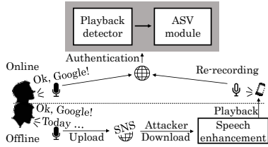
Figure 1. Playback spoofing attack using enhanced stolen speech method under ASVspooft 2017 scenario. Without speech enhancement, attack is the same as a conventional playback attack.
