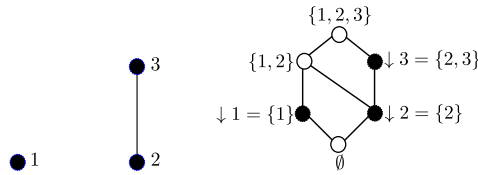
Fig. 2. Illustration of Birkhoff's Representation Theorem.
