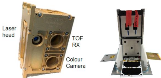
Figure 4. Left: Vision Based Navigation payload, Right: DS-2 target in deployed state
