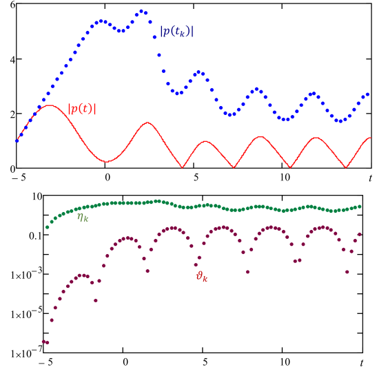
Figure 2. The results of simulation for (1) with t_0 = -5
