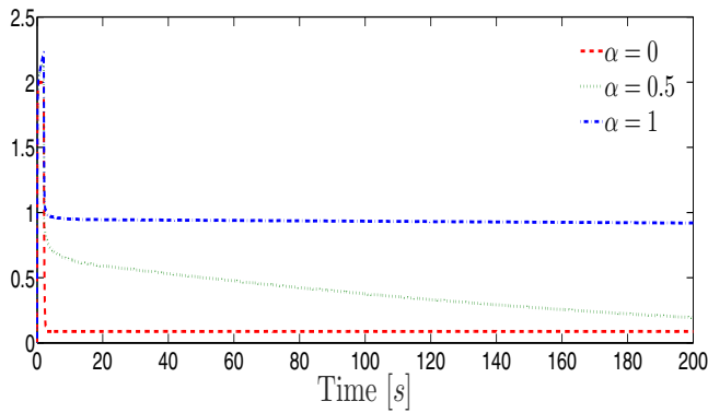
Figure 5. Estimation Error Index e_{RMS}(t) .
