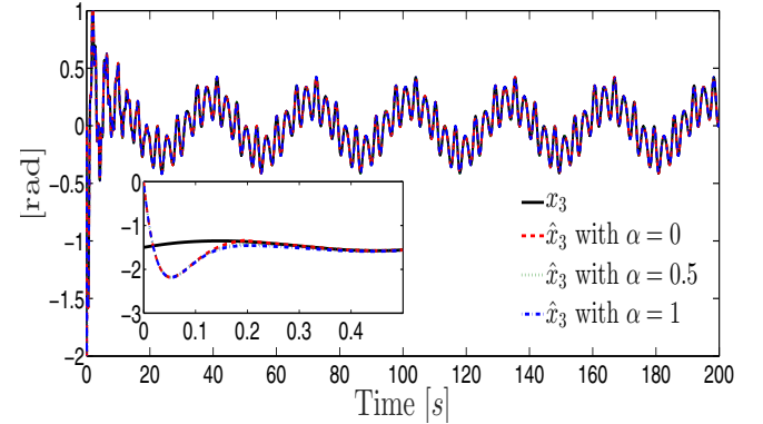
Figure 2. Estimation of x_3 .
