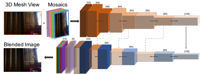
Fig. 8. DeepBlending network architecture. An RGB view of the global mesh is concatenated channel-wise with 4 RGB mosaic images and fed into a fully convolutional U-net-type architecture. Each successive block is generated via a 3 \times 3 convolution followed by a ReLU activation; the number of channels for each block is shown in brackets. Dotted lines represent “skip connections,” where features in the down-convolution portion are concatenated to features in the up-convolution portion. Decreases in spatial resolution are made by convolving with a stride of two, and increases use nearest-neighbor upsampling before the convolution is applied. A softmax activation is applied to obtain per-pixel blend weights. The novel image is obtained by taking the per-pixel weighted sum of the 5 network inputs.
