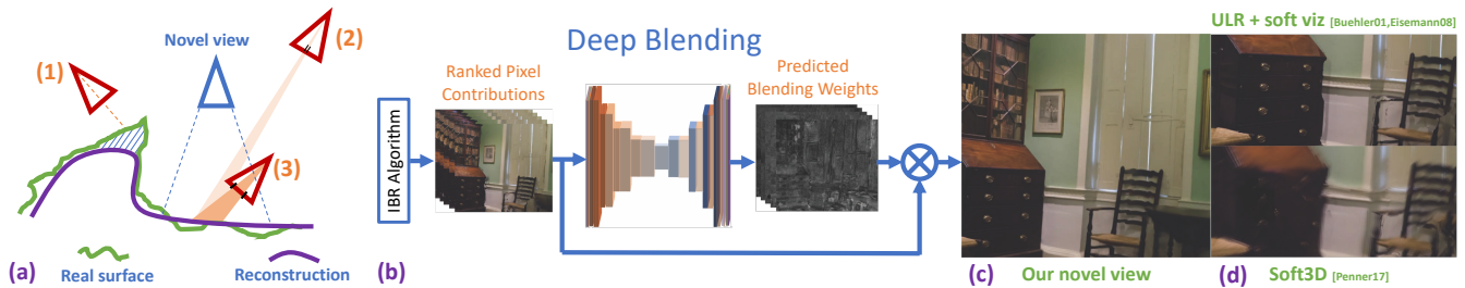
Fig. 1. Image-based rendering blends contributions from different input images to synthesize a novel view. (a) This blending operation is complex for a variety of reasons. For example, incorrect visibility ( e.g. , for the non-reconstructed green surface in input view (1)) may result in wrong projections of an image into the novel view. Blending must also account for, e.g. , differences in projected resolution ((2) and (3)). Previous methods have used hand-crafted heuristics to overcome these issues. (b) Our method generates a set of ranked contributions (mosaics) from the input images and uses predicted blending weights from a CNN to perform deep blending and synthesize (c) novel views. Our solution significantly reduces visible artifacts compared to (d) previous methods.
