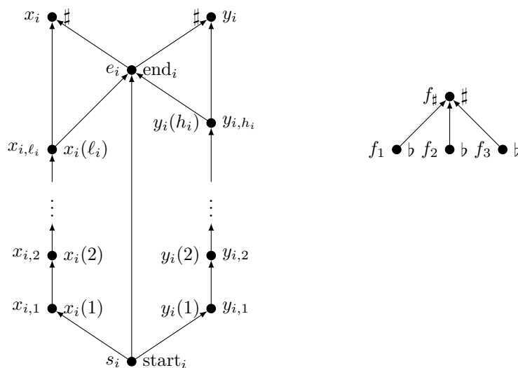
■ Figure 6 Templates T_i and T_\sharp .
