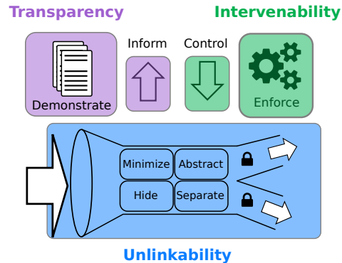
Fig. 4. Privacy Design Strategies
