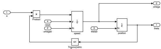
Figure 6. Simulink model of the pendulum
