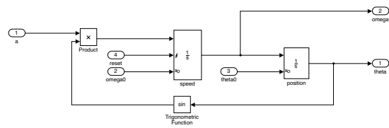
Figure 6. Simulink model of the pendulum
