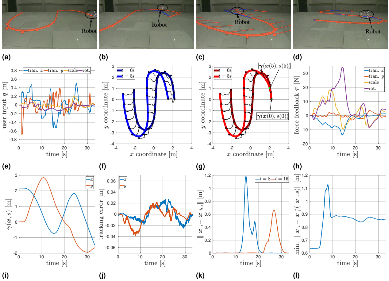
Figure 12. Experiment 1: open path. (a)-(d) Snapshots from the experiment with an overlay of the paths \gamma_S(x) (red) and \gamma_S(x_h) (blue). (a) Initial condition. (b) The path is being translated. (c) The path is being rotated. (d) The path is scaled down. (e) Input device's configuration q controlled by the user to give the commands. (f) Evolution of the desired path \gamma_S(x_h) in the first five seconds. The circles are the control points and the black lines show their trajectories. (g) Evolution of the desired path \gamma_S(x) in the first five seconds. The circles are the control points, the black lines show their trajectories and the green marker indicates the point \gamma(x(t), s(t)) tracked by the robot. (h) Force feedback. (i) Reference trajectory for the robot. (j) Robot's trajectory tracking error. (k) Mismatch \|x_i - x_{h,i}\| for individual control points. (l) Minimum distance from the singular curves.
