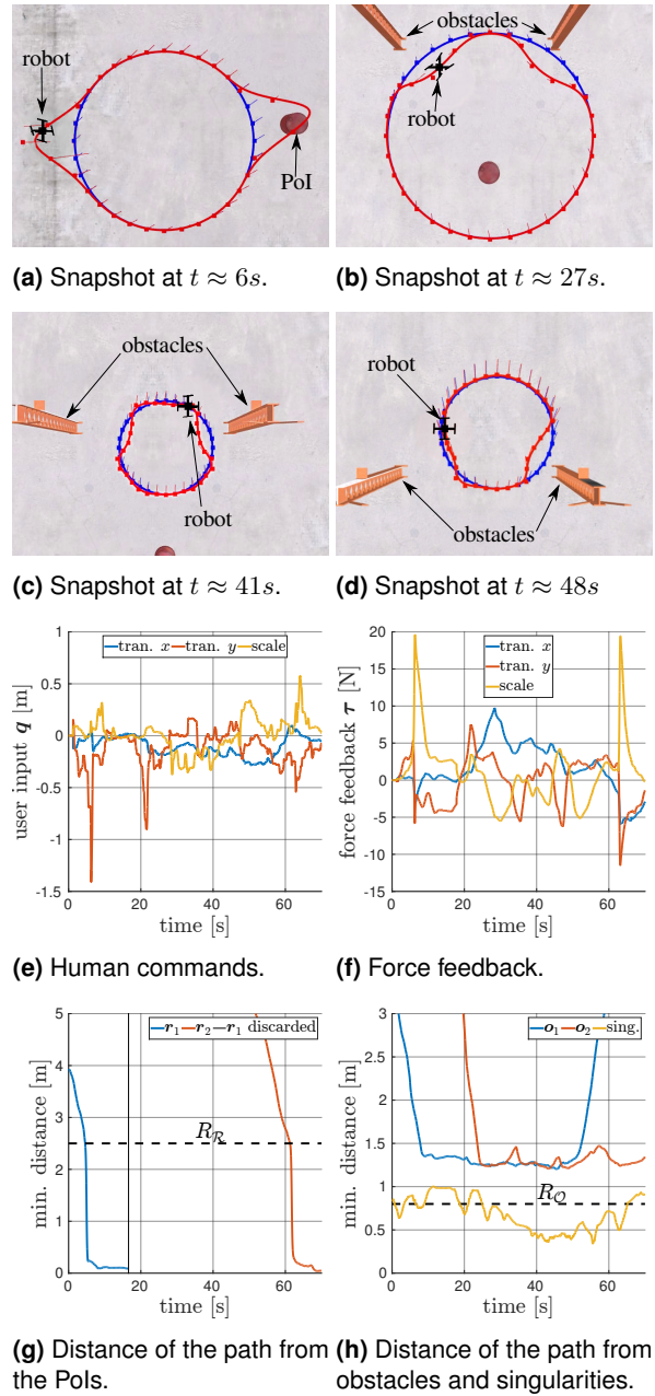
Figure 10. Simulation 2: obstacles and Pols (plots).
