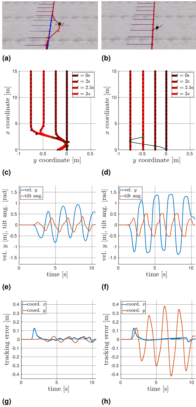
Figure 9. Simulation 1. (a), (c), (e), (g) refer to the case with N . (b), (d), (f), (h) refer to the case without N . (a) and (b): snapshots of the simulation showing \gamma_S(x_h) (blue thick line), \gamma_S(x) (red thick line), x_h (blue squares), x (red squares), \dot{x}_h (thin blue lines) and \dot{x} (thin red lines). (c) and (d): illustration of \gamma_S(x) in four moments. The reference position \gamma(x, s) in these moments is denoted by the green markers. The black line shows the reference trajectory followed by the robot. (e) and (f): lateral velocity and tilt angle of the robot. (g) and (h): tracking error (robot's position - reference position).
