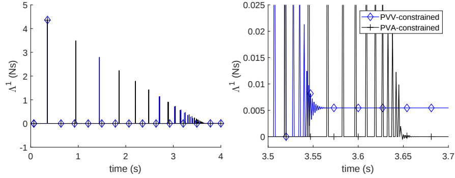
Fig. 7 Lagrange multiplier \tilde{\Lambda} of the bilateral constraint in the bouncing pendulum example (left: full time interval, right: zoom on the end phase).
