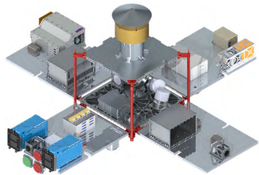
Fig. 4: Platform in Full Soft Stack Configuration. Panels are hinged open with the following subsystems. Centre panel: net payload. Bottom-left panel: 2 x CubeSats and deployer pods, antennas, first supervision camera. Top-left panel: harpoon target assembly payload, first card frame. Top-right panel: VBN payload, dragsail payload. Bottom-right panel: second card frame, second supervision camera.
