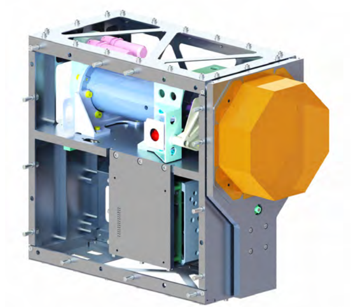
Fig. 20: Harpoon: Overall System including Target Assembly Showing: harpoon chamber and mountings (blue, cyan), CGGs (pink), frangibolt (red), OSS boom unit (green), Kapton box (yellow).
