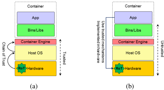
Figure 1: Different scenarios of trusted execution of containers.
