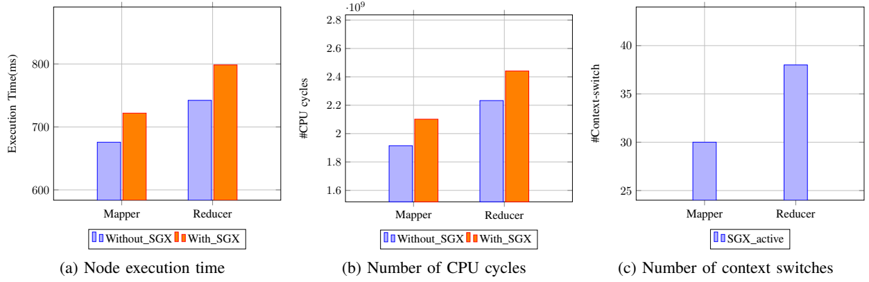
Figure 4: Performance of Mapper and Reducer nodes with and w/o Intel SGX.
