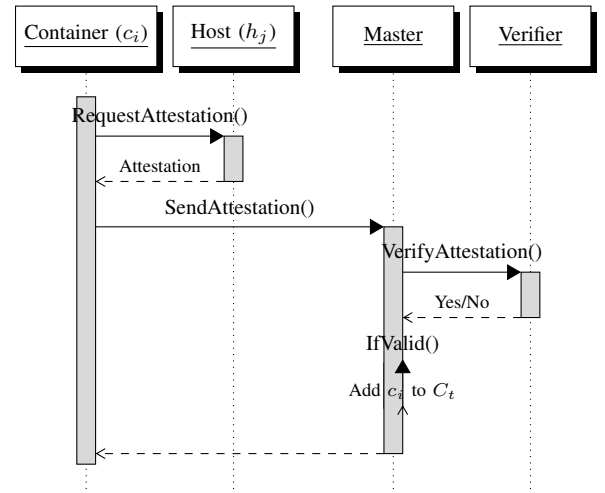
Figure 3: Join protocol: adding a container to a trusted cluster.
