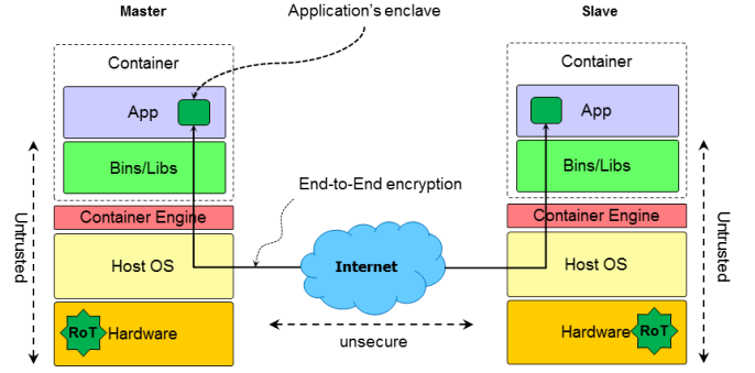
Figure 2: End-to-end encryption between two enclaves.
