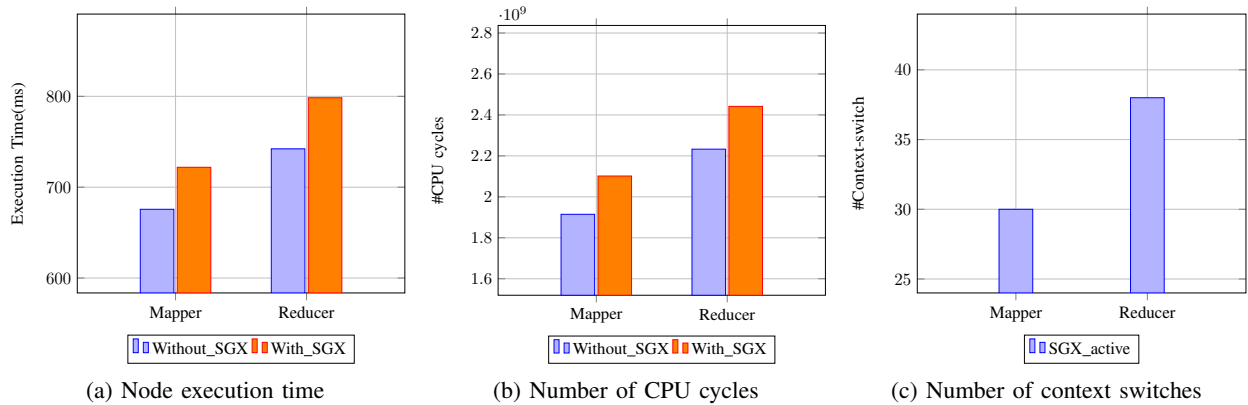
Figure 4: Performance of Mapper and Reducer nodes with and w/o Intel SGX.
