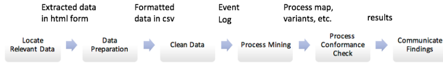
Fig. 2. The methodology followed in this article for process conformance check
