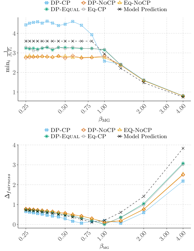
Figure 9: Minimum throughput and \Delta_{fairness} for CG and MG, where both applications have six cores.
