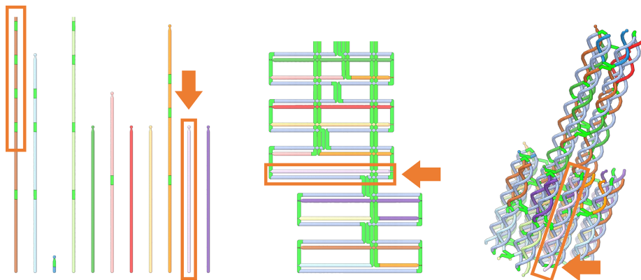
Figure 9: DNA nanotube in 1D, 2D and 3D [45]. Crossovers are highlighted in green.
