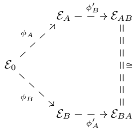
Fig. 2. Supersingular Isogeny Diffie–Hellman.
