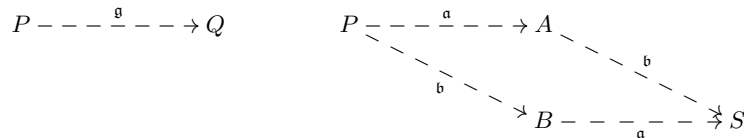
Fig. 1. Vectorization (left: finding the unique \mathfrak{g} such that Q = \mathfrak{g} \cdot P ) and parallelization (right: computing the unique S such that S = \mathfrak{g}_B \cdot A = \mathfrak{g}_A \cdot B = (\mathfrak{g}_A \mathfrak{g}_B) \cdot P ). The dashed arrows denote actions of the unknown group elements \mathfrak{g} , \mathfrak{g}_A , and \mathfrak{g}_B .
