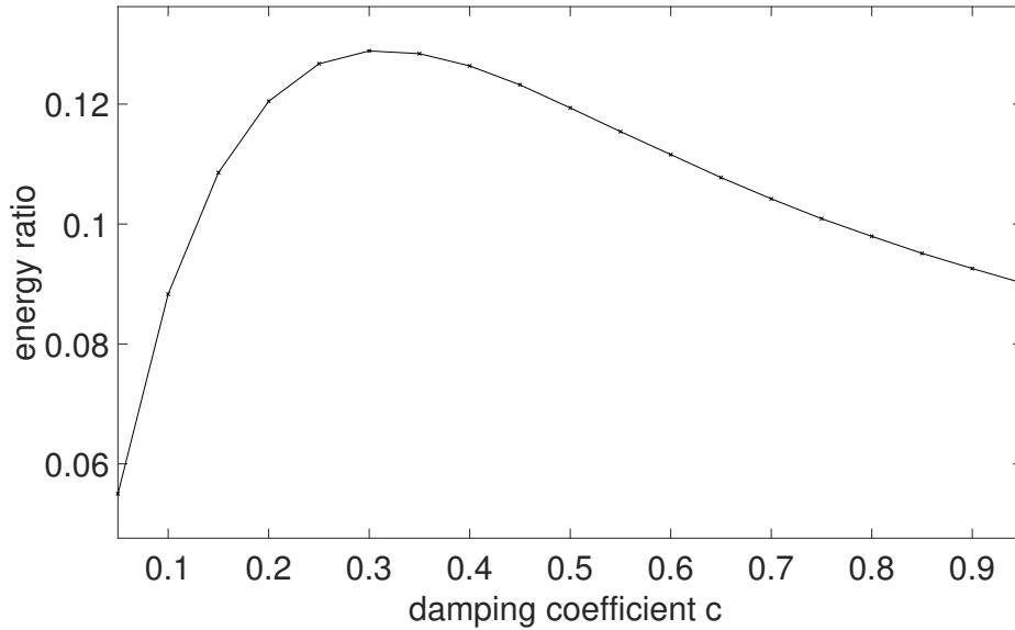
FIGURE 8. Spring: energy ratio for different values of the damping coefficient
