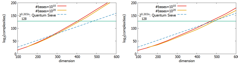
Fig. 1. Q-sieve vs Q-enum: (Left) Using HKZ bases (Right) Using Rankin bases
