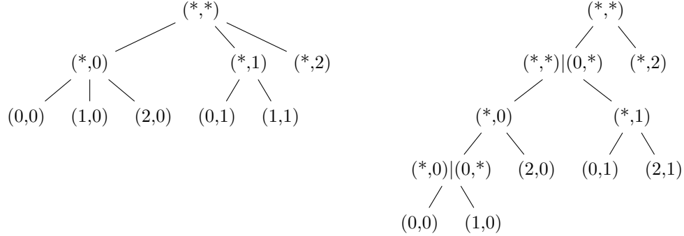
Fig. 3. An example of the transformation in Th. 5
