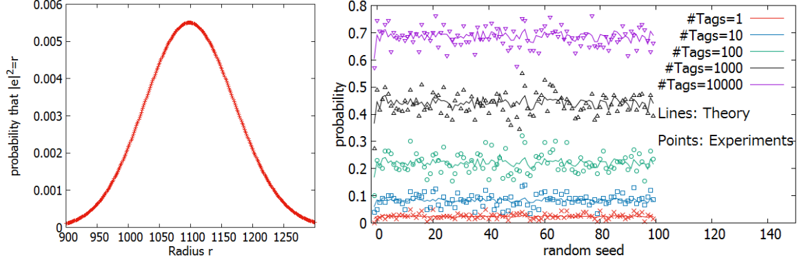
Fig. 6. (Left) The graph of \Pr_e[\|\mathbf{e}\|^2 = r^2] for GGH-200's noise; (Right) Theoretical and experimental success probability on PBKZ-60 bases of the GGH-200 lattice.
