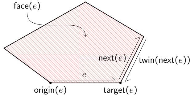
Figure 4. Atomic functions applied to a face in the mesh. For any half-edge e of the face it is true that the half-edge e' = \text{edge}(\text{face}(e)) belongs to the face, too.
