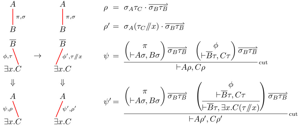
Figure 6: The critical pair \vdash A, B ; \vdash \overline{B}, \exists x.C
