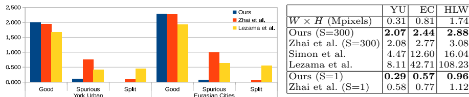
Fig. 7. Left: performance results w.r.t. VP detection. Right: computation times in sec.
