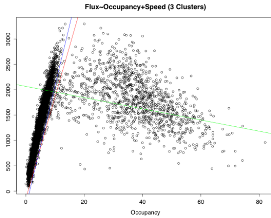
Figure 15: Flux Vs Occupancy+Speed: RSS analysis
