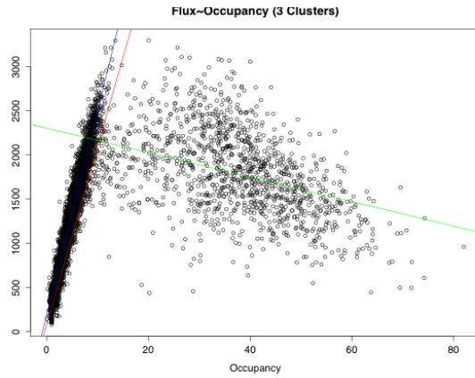
Figure 14: Flux Vs Occupancy: RSS analysis
