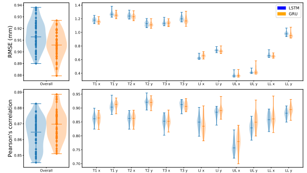
Figure 3: Violin plot for RMSE (mm) and Pearson's correlation of 50 independent training using either LSTM or GRU units. Subplots on the right correspond to performances per coils, and subplots on the left correspond to the overall performances. Each dot corresponds to a single training.
