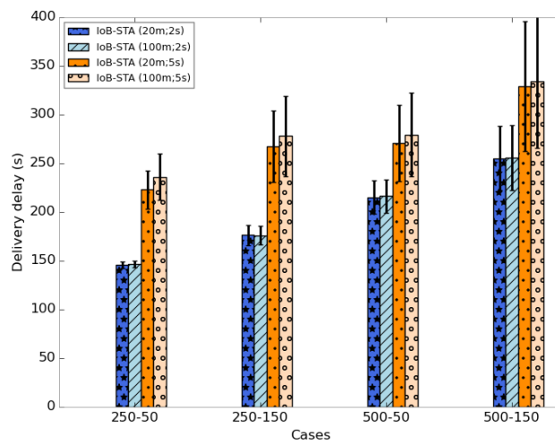
Figure 36. Average delivery delay for IoB-STA.
