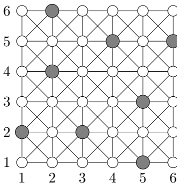
Figure 1: Tile generating an optimal identifying code of the infinite king grid. Black vertices are those of the code.
