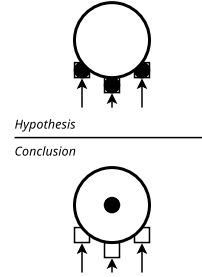
Fig. 4: Illustration of the rule of Equation (3) to move tokens from input docks to a place.
