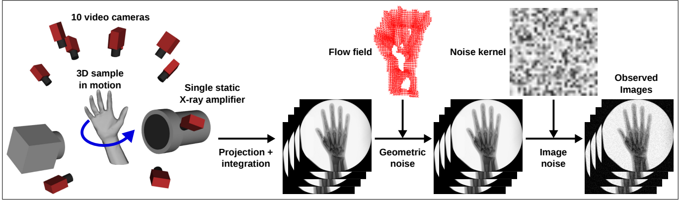
Fig. 2. X-ray image formation model for a moving sample observed by a single static planar X-ray amplifier. Video cameras are used to recover the sample surface motion. The formation model is composed of 3D attenuation projection and integration into a 2D image, geometric noise, and image noise.
