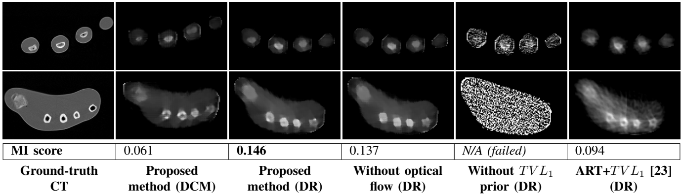
Fig. 16. Results on the forearm phantom: 2 selected slices and Mutual Information (MI) score for both DR and DCM datasets. MI registration scores are provided for quantitative comparison with differing pose/spectrum parameters. Without optical flow, artefacts are visible, for example in the bone cavities. The ART+ TVL_1 method produces much noisier results with obvious streak artefacts due to under-sampling. We also observe that the DCM dataset produces slightly noisier and sharper reconstructions compared to the DR dataset with the proposed method. The MI score for the proposed method (DCM) is lower than that for ART+ TVL_1 (DR), however these scores are not to be compared directly as both the dataset and the method differ in these two results.
