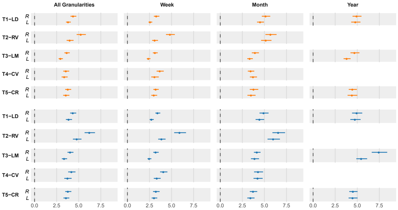
Fig. 2. Mean Completion Times in seconds for tasks 1-5 with R adial and L inear layouts. Task abbreviations: T1-LD = L ocate D ate, T2-RV = R ead V alue, T3-LM = L ocate M in / M ax, T4-CV = C ompare V alues, T5-CR = C ompare R anges. ● = Temperature; ● = Sleep. As indicated in Table 1, T2 and T4 did not include trials at the Year level. Error bars are 95% CIs; for guidance with respect to interpreting overlaps in CIs, refer to [40].
