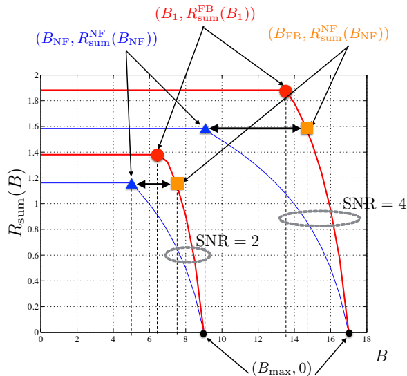
Fig. 6. Information sum-capacity of the symmetric two-user memoryless G-MAC-F(0) (thick red line) and G-MAC(0) (thin blue line), with co-located receiver and EH, with \text{SNR}_{11} = \text{SNR}_{12} = \text{SNR}_{21} = \text{SNR}_{22} = \text{SNR} , as a function of B . Red (big) circles represent the pairs (B_1, R_{\text{sum}}^{\text{FB}}(B_1)) in which R_{\text{sum}}^{\text{FB}}(B_1) is the information sum-capacity with feedback when only information transmission is performed and B_1 \triangleq 1 + 2(1 + \rho^*(1, 1))\text{SNR} represents the corresponding maximum energy rate that can be guaranteed at the EH. Blue triangles represent the pairs (B_{\text{NF}}, R_{\text{sum}}^{\text{NF}}(B_{\text{NF}})) in which R_{\text{sum}}^{\text{NF}}(B_{\text{NF}}) is the information sum-capacity without feedback and B_{\text{NF}} \triangleq 1 + 2\text{SNR} is the corresponding maximum energy rate that can be guaranteed at the EH without feedback. Orange squares represent the pairs (B_{\text{FB}}, R_{\text{sum}}^{\text{NF}}(B_{\text{FB}})) in which B_{\text{FB}} is the corresponding maximum energy rate that can be guaranteed at the EH with feedback. Black (small) circles represent the pairs (B_{\text{max}}, 0) in which B_{\text{max}} \triangleq 1 + 4\text{SNR} is the maximum energy rate at the EH.
