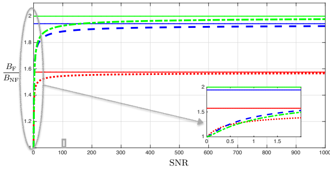
Fig. 7. The ratio \frac{B_{\text{FB}}}{B_{\text{NF}}} and its high-SNR limit as a function of SNR when the receiver and the EH are co-located and \text{SNR}_{11} = \text{SNR}_{21} = \text{SNR}_1 and \text{SNR}_{12} = \text{SNR}_{22} = \text{SNR}_2 . The solid line is the high-SNR limit in (50); the dash-dotted line, the dashed line and the dotted line are the exact values of the ratio \frac{B_{\text{FB}}}{B_{\text{NF}}} in (48) when \text{SNR}_1 = \text{SNR}_2 = \text{SNR} ; \frac{\text{SNR}_1}{2} = \text{SNR}_2 = \text{SNR} ; and \frac{\text{SNR}_1}{10} = \text{SNR}_2 = \text{SNR} , respectively.
