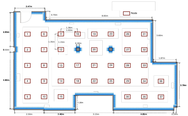
Figure 2: R2lab topology
