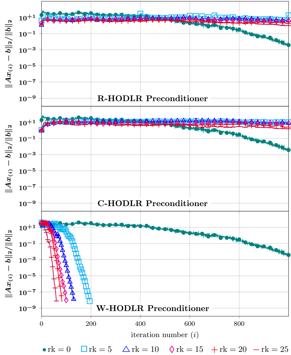
Figure 6: PCG Convergence History: 'bcsstk15'. Three plots showing PCG convergence history profiles, i.e., the values \|Ax_{(i)} - b\|_2 / \|b\|_2 as a function of the iteration number i , for each preconditioning scheme. Each plot displays various profiles, where each profile corresponds to a different constant rank value eq. (4.1) of the approximations for the off-diagonals blocks by low-rank factorizations.
