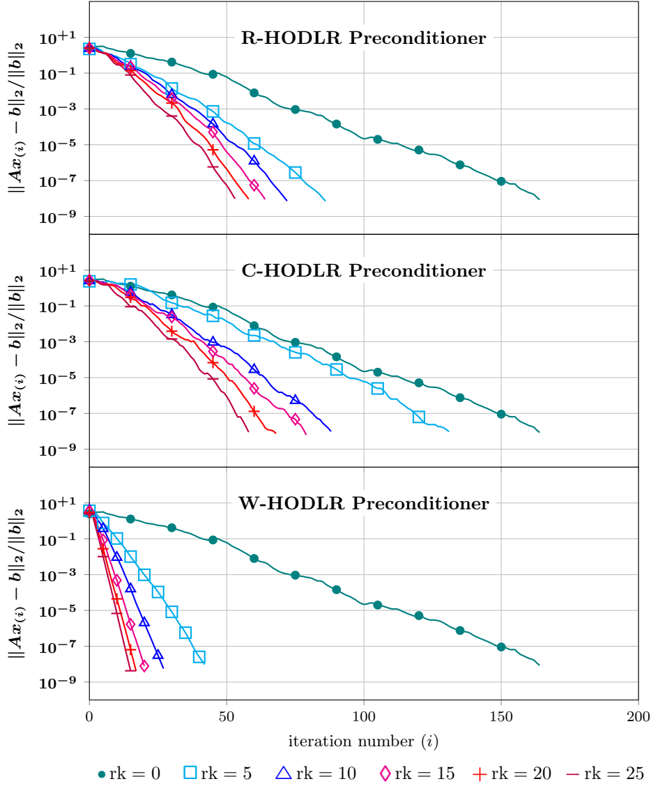
Figure 5: PCG Convergence History: 'bcsstk16' . Three plots showing PCG convergence history profiles, i.e., the values \|Ax_{(i)} - b\|_2 / \|b\|_2 as a function of the iteration number i , for each preconditioning scheme. Each plot displays various profiles, where each profile corresponds to a different constant rank value eq. (4.1) of the approximations for the off-diagonals blocks by low-rank factorizations.
