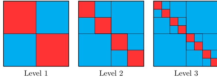
Figure 2: The HODLR Structure. The first 3 levels, \ell = 1, 2, 3 , of the HODLR structure are illustrated: at each level the blue color blocks are the low-rank off-diagonal blocks and the red blocks are the HODLR principal submatrices.
