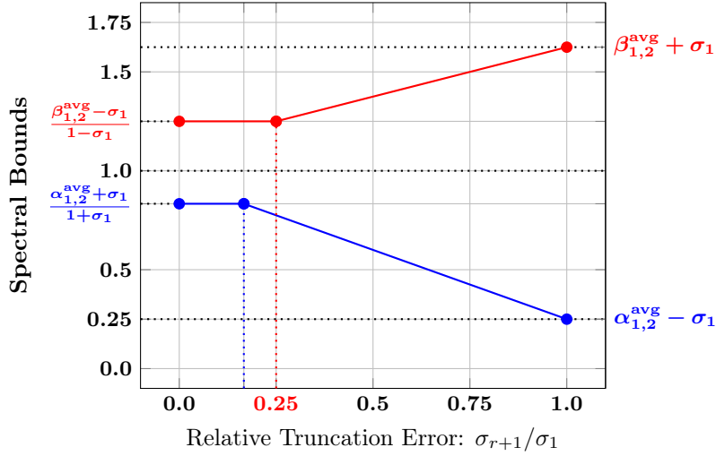
Figure 3: Spectral Bounds. A typical behavior of the spectral bounds displayed for the case \alpha_1 = \alpha_2 and \beta_1 = \beta_2 . The lower bound \alpha eq. (3.13) vs. \sigma_{r+1}/\sigma_1 is plotted in blue, and the upper bound \beta eq. (3.14) vs. \sigma_{r+1}/\sigma_1 is plotted in red.
