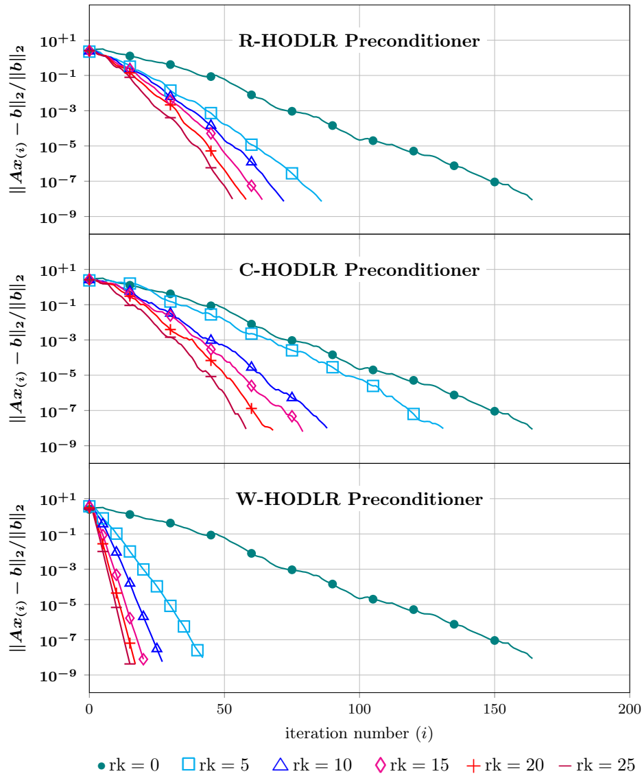
Figure 5: PCG Convergence History: 'bcsttk16' . Three plots showing PCG convergence history profiles, i.e., the values \|Ax_{(i)} - b\|_2 / \|b\|_2 as a function of the iteration number i , for each preconditioning scheme. Each plot displays various profiles, where each profile corresponds to a different constant rank value eq. (4.1) of the approximations for the off-diagonals blocks by low-rank factorizations.
