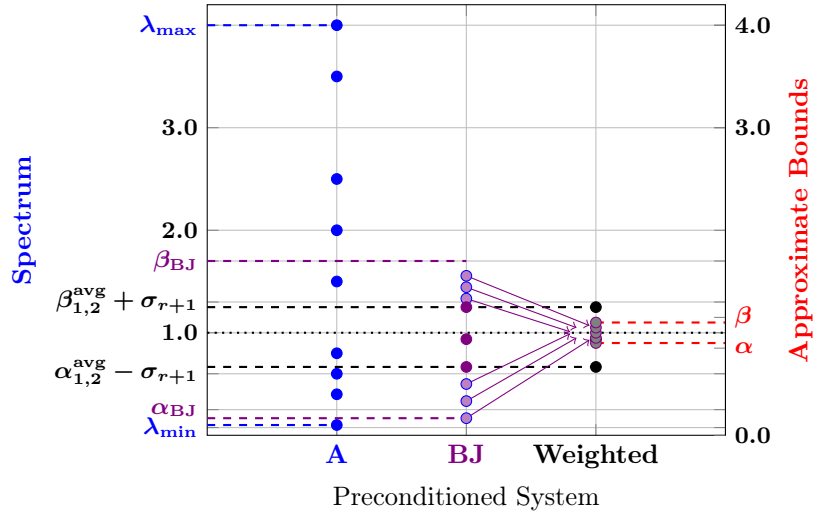
Figure 4: Spectrum Clustering for the Multilevel Weighted HODLR Preconditioning Scheme. The spectrum of some SPD matrix A and the transformation it goes after preconditioning by block Jacobi (BJ) and the multilevel weighted HODLR preconditioning scheme are displayed. The spectra are ordered from the left to the right starting from A , followed by Block Jacobi (BJ) and ends up with the multilevel weighted HODLR scheme. The spectral bounds \alpha eq. (3.13) and \beta eq. (3.14) are marked on the right y -axis, while the spectral bounds for the block Jacobi case \alpha_{\text{BJ}} = \alpha(r = 0) and \beta_{\text{BJ}} = \beta(r = 0) are marked on the left y -axis.
