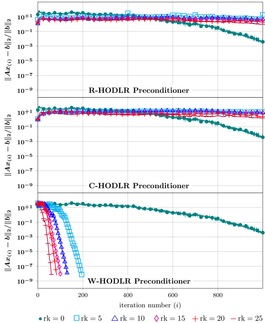
Figure 6: PCG Convergence History: 'bcsstk15' . Three plots showing PCG convergence history profiles, i.e., the values \|Ax_{(i)} - b\|_2 / \|b\|_2 as a function of the iteration number i , for each preconditioning scheme. Each plot displays various profiles, where each profile corresponds to a different constant rank value eq. (4.1) of the approximations for the off-diagonals blocks by low-rank factorizations.
