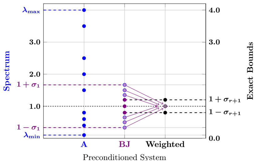
Figure 1: Spectrum Clustering of the Optimal 1-level Preconditioning Scheme. The spectrum of some SPD matrix A and the transformations it goes after preconditioning by block Jacobi (BJ) and the optimal 1-level preconditioning scheme are displayed. The spectra are ordered from the left to the right starting from A , followed by BJ and end up with the optimal scheme.
