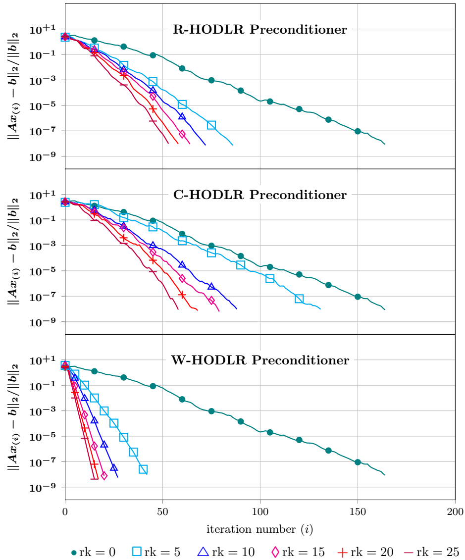
Figure 9: PCG Convergence History: 'bcsttk16' . Three plots showing PCG convergence history profiles, i.e., the values \|Ax_{(i)} - b\|_2 / \|b\|_2 as a function of the iteration number i , for each preconditioning scheme. Each plot displays various profiles, where each profile corresponds to a different constant rank value eq. (4.6) of the approximations for the off-diagonals blocks by low-rank factorizations.
