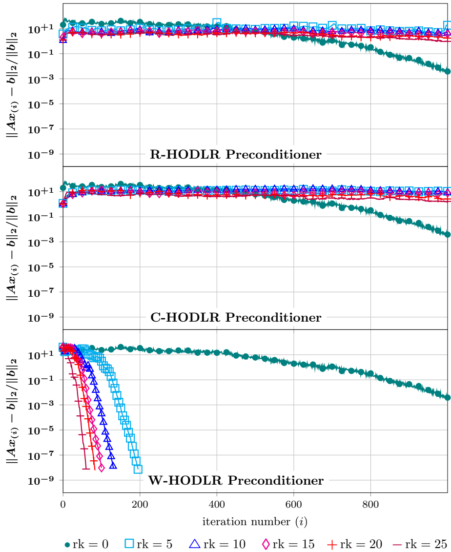
Figure 10: PCG Convergence History: 'bcstk15' . Three plots showing PCG convergence history profiles, i.e., the values \|Ax_{(i)} - b\|_2 / \|b\|_2 as a function of the iteration number i , for each preconditioning scheme. Each plot displays various profiles, where each profile corresponds to a different constant rank value eq. (4.6) of the approximations for the off-diagonals blocks by low-rank factorizations.
