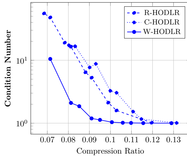
Figure 6: Condition Number vs. Compression: 'Subdomain1000' . Each plot shows the condition number achieved by an HODLR preconditioned system as a function of the compression ratio.
