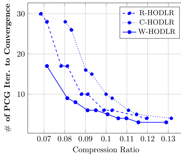
Figure 7: Iterations to Convergence vs. Compression: 'Subdomain1000' . Each plot shows the number of PCG iterations to convergence achieved by each HODLR preconditioned system as a function of the compression ratio.
