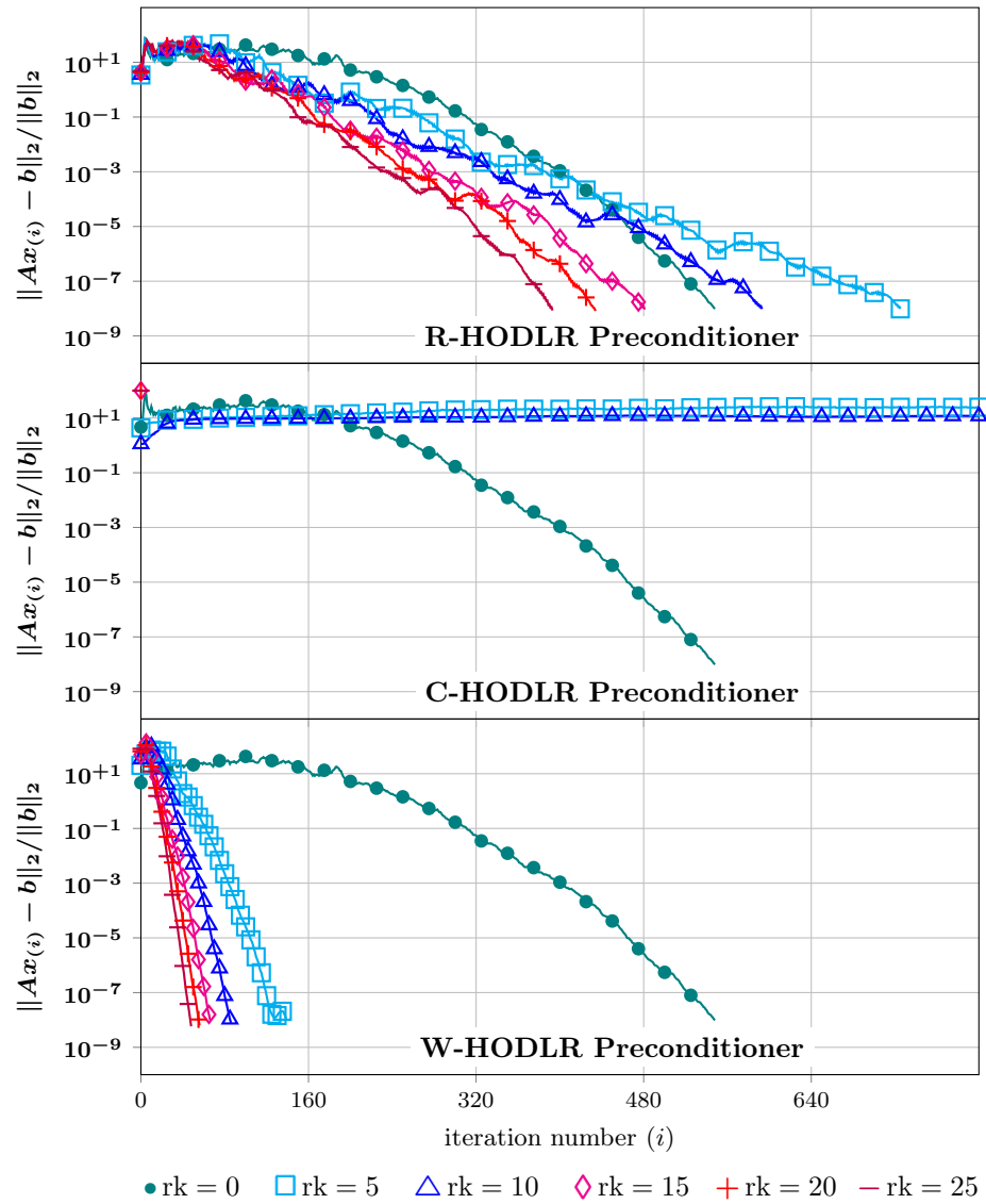
Figure 11: PCG Convergence History: 'SparseRob500' . Three plots showing PCG convergence history profiles, i.e., the values \|Ax_{(i)} - b\|_2 / \|b\|_2 as a function of the iteration number i , for each preconditioning scheme. Each plot displays various profiles, where each profile corresponds to a different constant rank value eq. (4.6) of the approximations for the off-diagonals blocks by low-rank factorizations.
