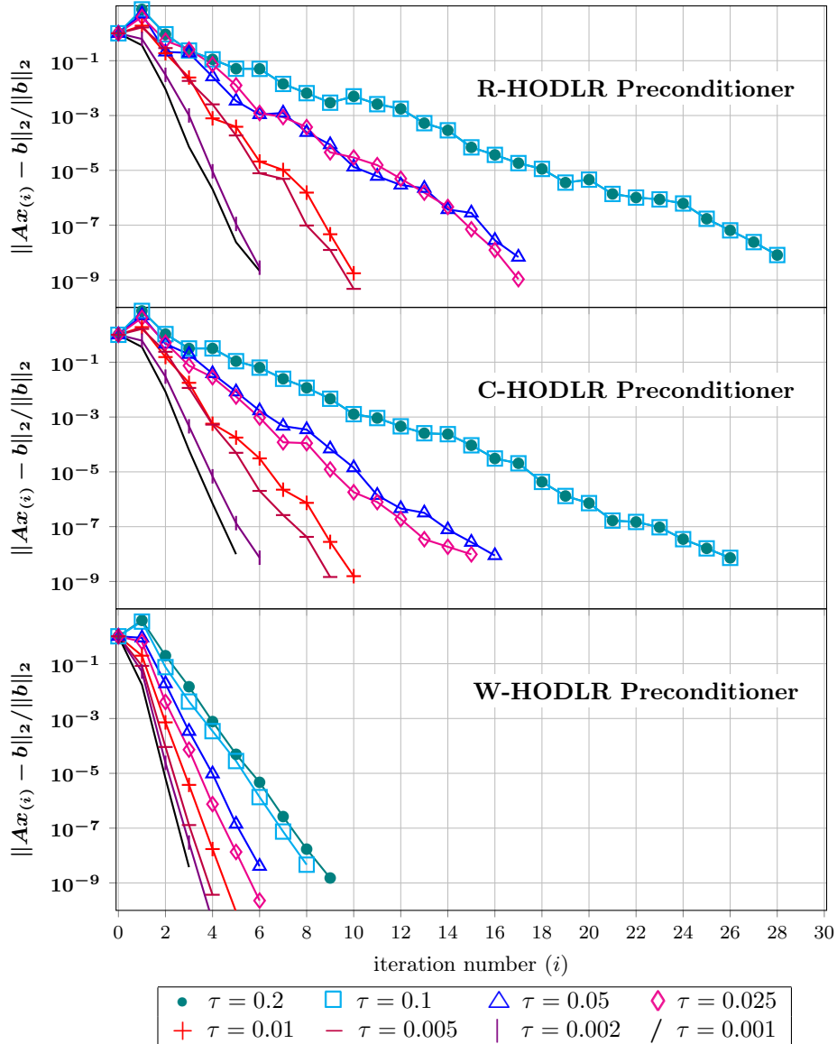
Figure 8: PCG Convergence History: 'Subdomain1000' . Three plots showing PCG convergence history profiles, i.e., the values \|Ax_{(i)} - b\|_2 / \|b\|_2 as a function of the iteration number i , for each preconditioning scheme. Each plot displays various profiles, where each profile corresponds to a different value eq. (4.4) of the uniform tolerance \tau that is employed to set the off-diagonal blocks approximations by low-rank factorizations.
